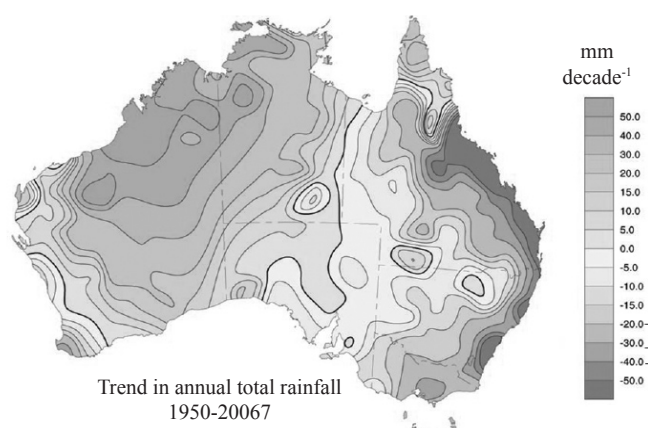
Figure 2a: Historical changes in mean annual rainfall for Australia over the period 1950-2007
