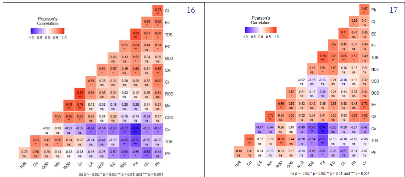
Figure 16; 17: Correlation matrix among different groundwater quality parameters in pre-monsoon and post-monsoon season; PH: pH; EC: Electrical conductivity; TUR: Turbidity; TDS: Total dissolved salts; CA: Calcium; CL: Chloride; NO 3 : Nitrate; BOD: Biological oxygen demand; COD: Chemical oxygen demand; Fe: Iron; Pb: Lead; Cr: Chromium; Cu: Copper; Mn: Manganese; ns: non-significant
