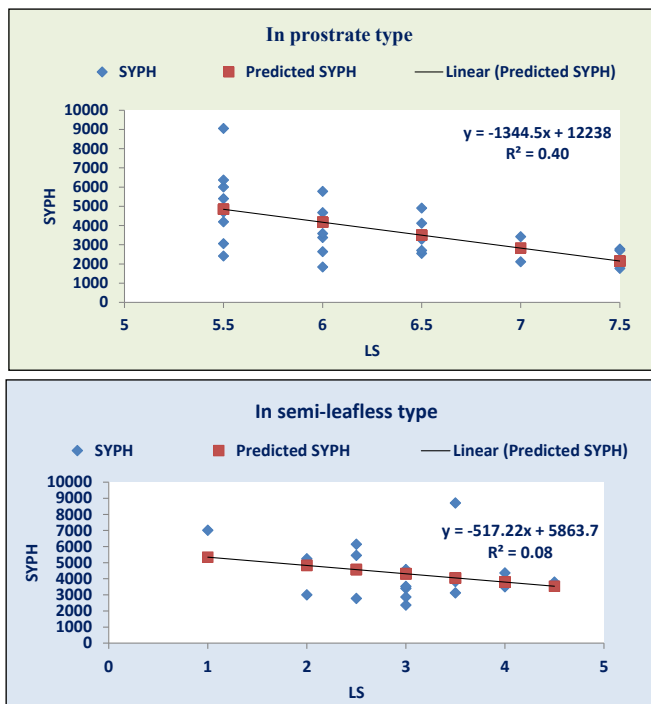
Figure 10: Seed yield in kg ha -1 vs. lodging severity score in prostrate/normal leafed and semi-leafless type field pea genotypes line fit plot by regression analysis
