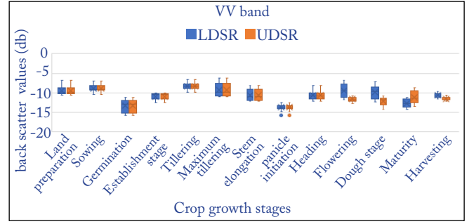
Figure 5: Graph showing spectral backscattering values
