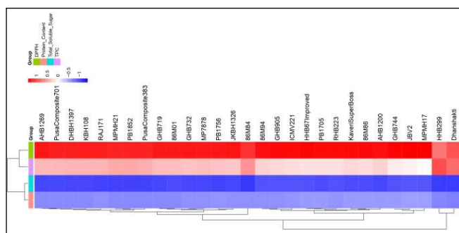
Figure 4: Heat map and double dendrogram representing expression pattern of proteins content, total soluble sugar, total phenolic contents and DPPH in pearl millet germplasms
