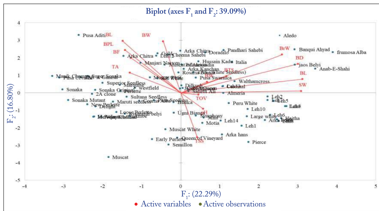
Figure 2: PCA biplot of 83 grape genotypes for quantitative fruits traits
