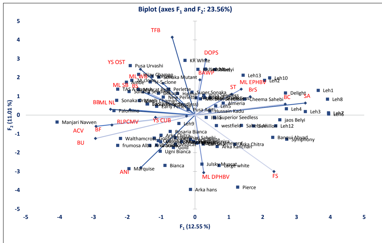
Figure 1: PCA biplot of 83 grape genotypes for qualitative morphological traits
