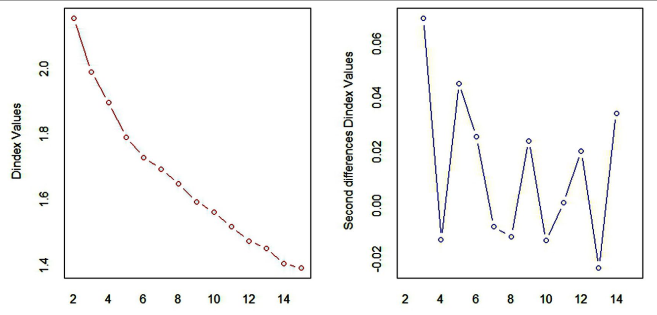
Figure 1: Graphical representation of the Dindex indicating the optimal number of clusters for 130 sugarcane genotypes: (a) Dindex values and (b) second difference of Dindex values
